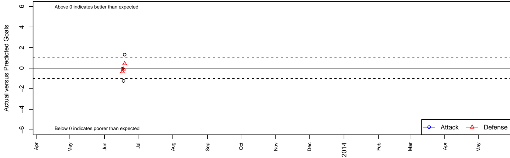
Colorado United White B96 Dots are actual minus expected GF (blue circles) and GA (red triangles). Blue line is smoothed change in attack strength. Red is smoothed change in defense strength.
